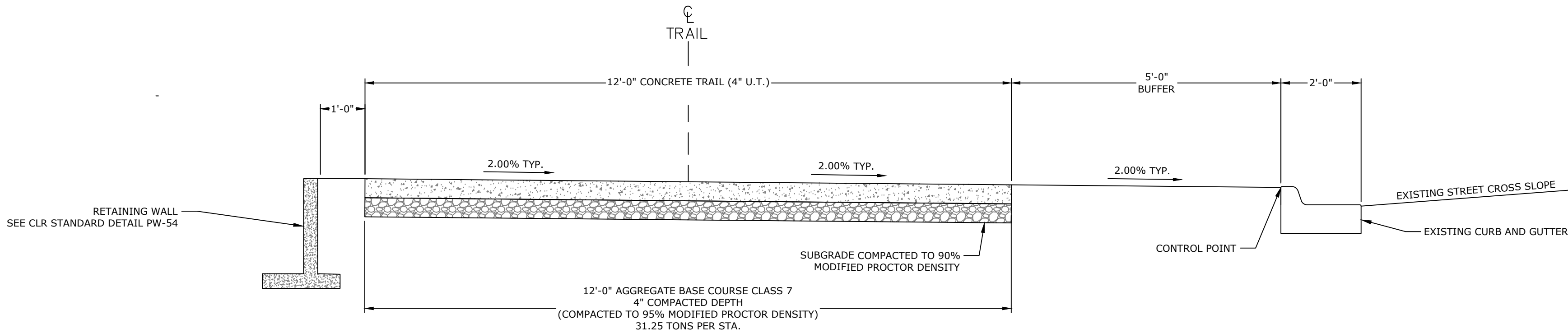
TRAIL WITH 5' BUFFER ON PROPOSED BACK OF CURB DETAIL (WITH GUTTER) N.T.S.
