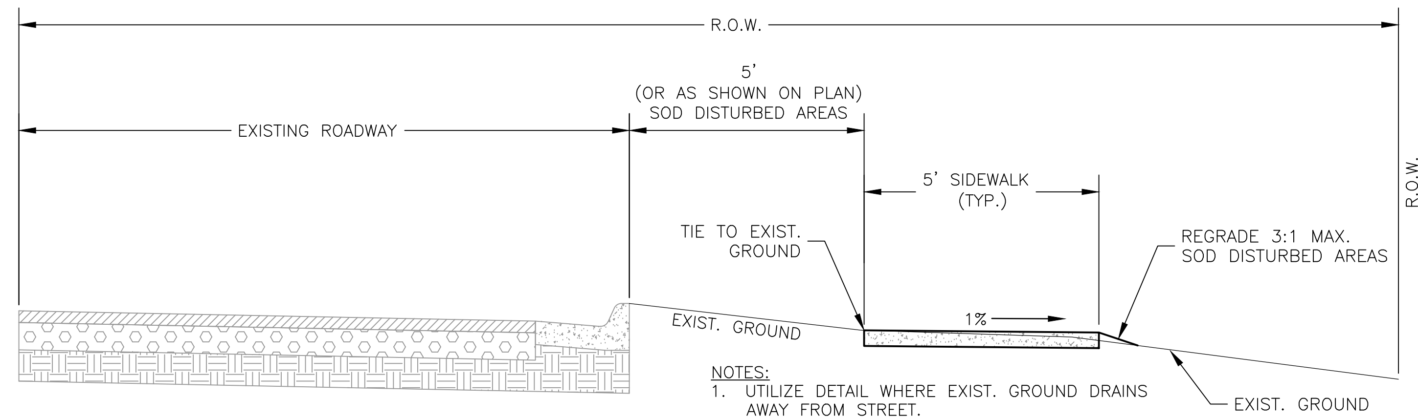
SIDEWALK DRAINING AWAY FROM STREET NTS
