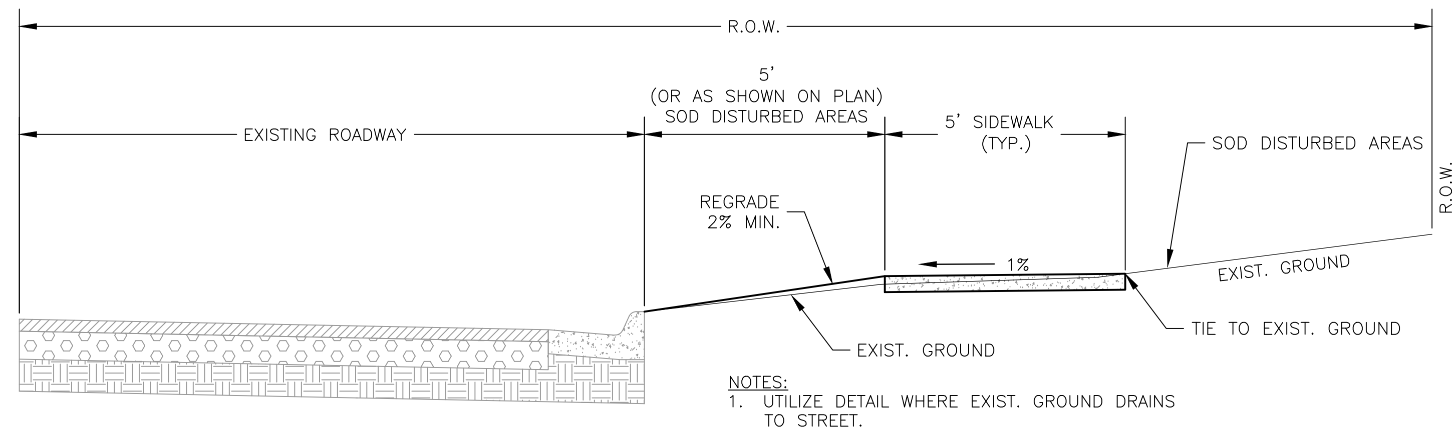
SIDEWALK DRAINING TO STREET NTS
