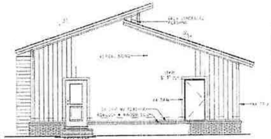
REAR ELEVATION
