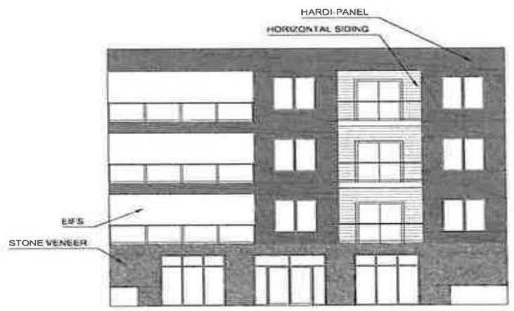
PARTIAL ENTRY ELEVATION 4-STORY BUILDING ————— SCALE: 1/8" = 1'-0"
