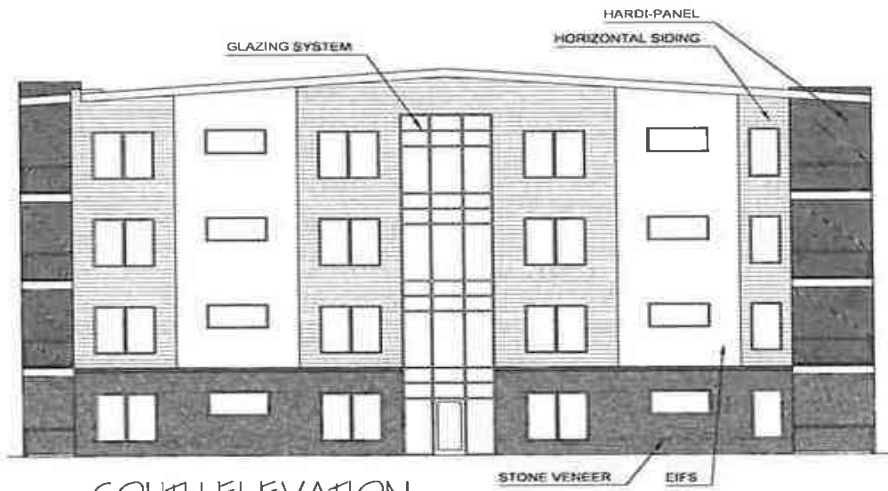
SOUTH ELEVATION 4-STORY BUILDING ————— SCALE: 1/8" = 1'-0"
