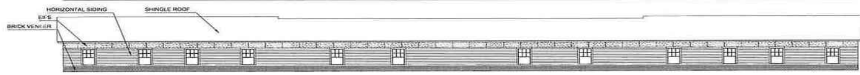
( 4 ) -2BR / ( 4 ) -1 BR / ( 0 ) -GARAGE REAR ELEVATION ————— SCALE: 1/ 8" =1'-0"
