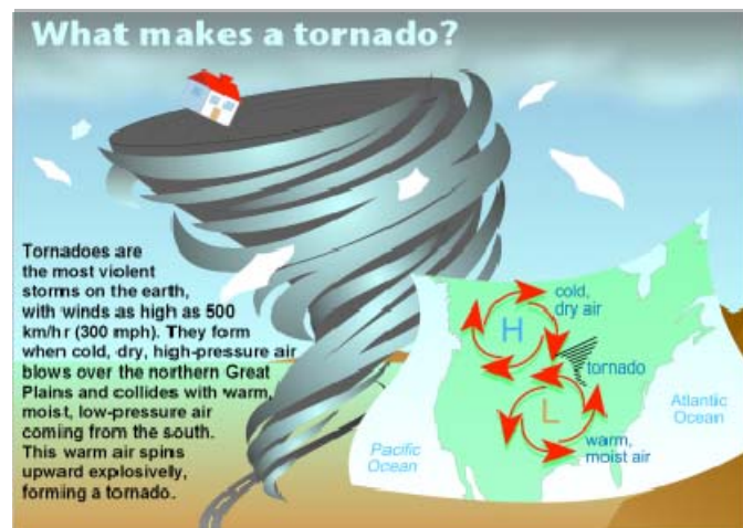
Figure 3.1 Precipitating Factors for a Tornado
