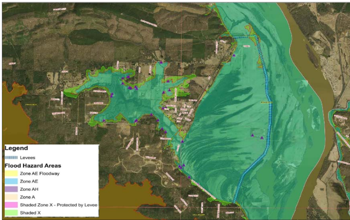
Figure 3.51 Roland Levee
