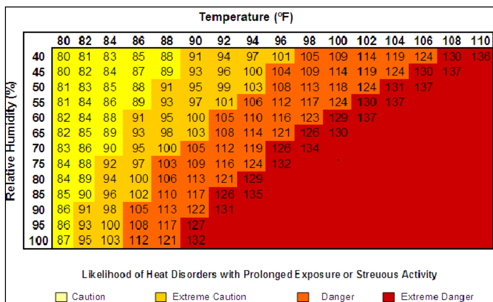
Figure 3.19 Heat Index
