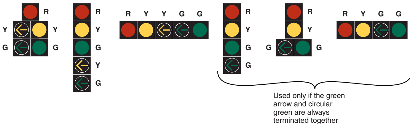
B - Typical arrangements
